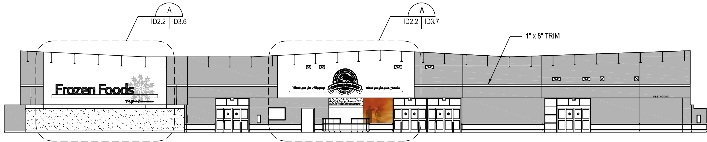
ELEVATION A ID1.2 | ID2.2 1/16"=1'-0"
